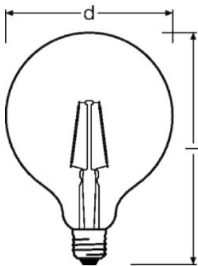
P RF CLAS GL 2.5 W/827 E27, P RF GLOBE 25 2 W/827 E27 FIL
