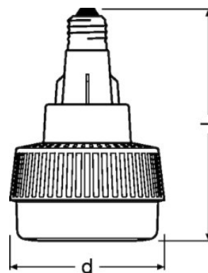
HQL LED PRO 95 W/840 E40
