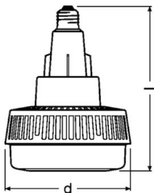
HQL LED PRO 95 W/840 E40, HQL LED PRO 140 W/840 E40, HQL LED PRO 140 W/840 E40
