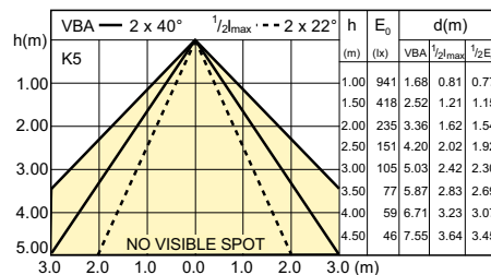
SDBE_LEDspotL_0134-Beam diagram
