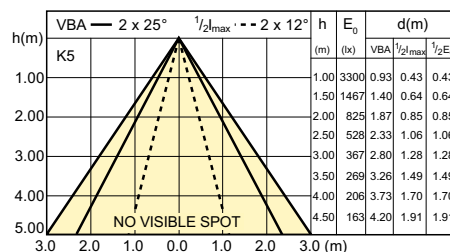
SDBE_LEDspotL_0137-Beam diagram
