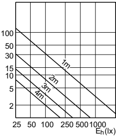
SDAC_LEDspotL_0137-Accent diagram
