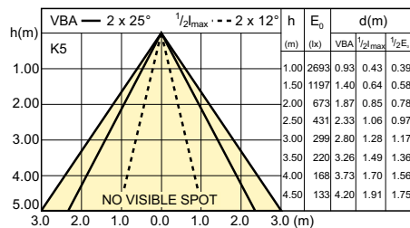
SDBE_LEDspotL_0133-Beam diagram
