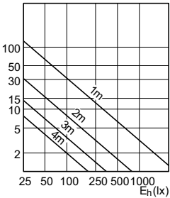
SDAC_LEDspotL_0136-Accent diagram
