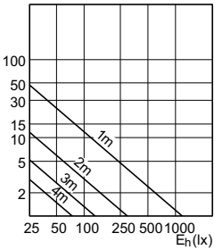
SDAC_LEDspotL_0135-Accent diagram
