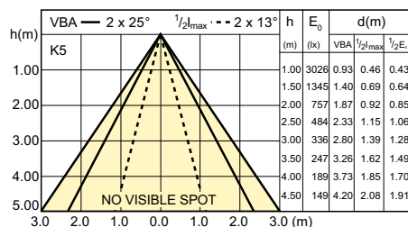
SDBE_LEDspotL_0136-Beam diagram
